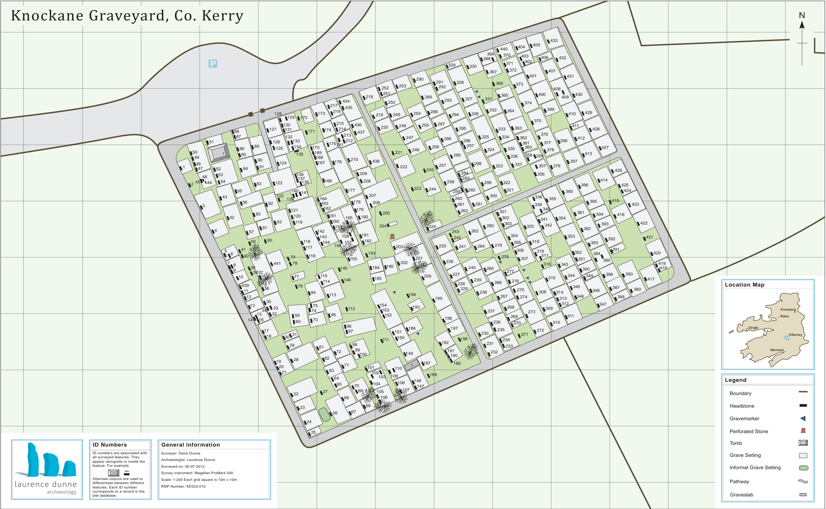
Figure 2: Archaeological survey plan of Knockane graveyard.
